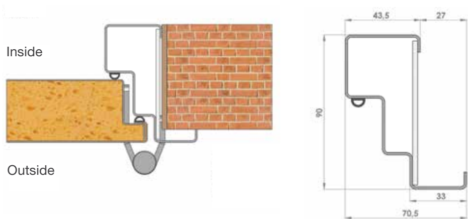
MITRED FRAME, OPEN TO OUTSIDE (LO)
