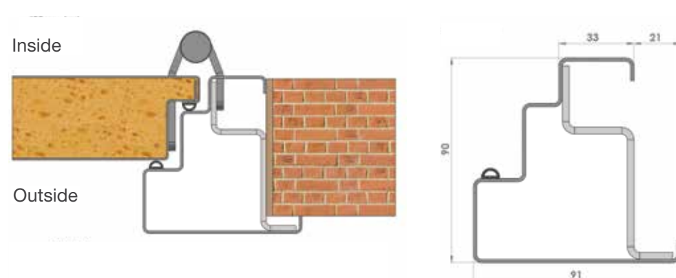
MITRED FRAME WITH MOULDINGS, OPEN TO INSIDE (MI)
